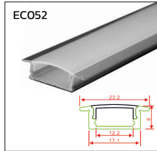
17mm SLIM CONCEALED
