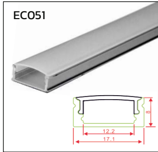
17mm SLIM SURFACE
